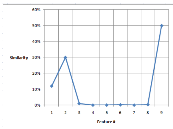
Fig. 2. Similarity of features of the attack
